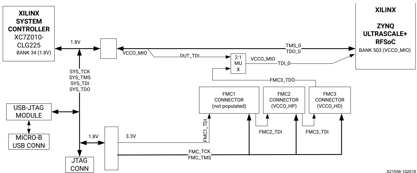
Figure 1-8: JTAG Chain
